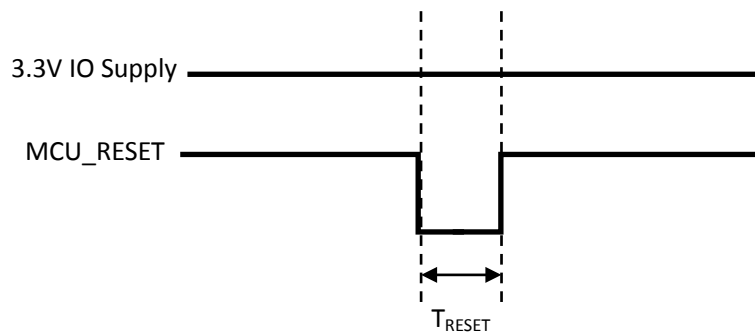
Figure 5-4-1: MCU Reset Timing
