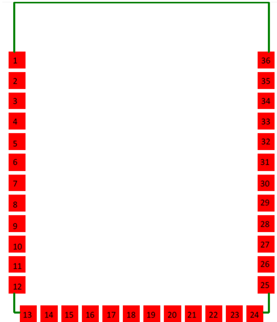
Figure 4-1-1: Module Pins Map
