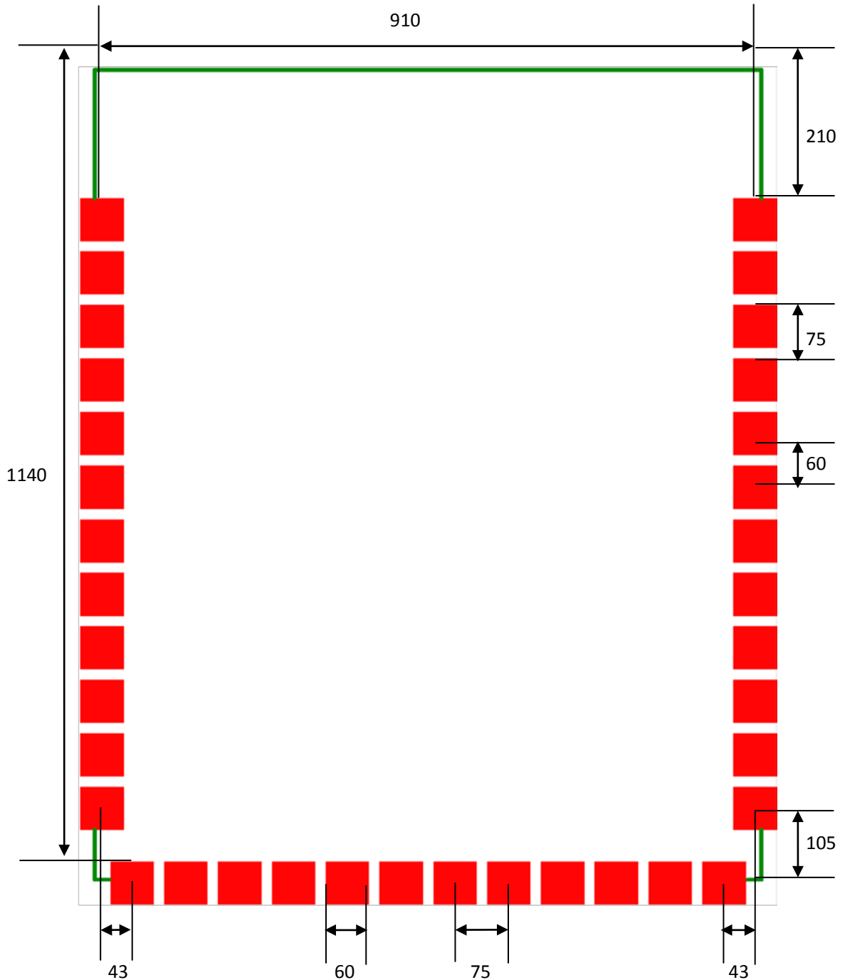
Figure 3-1-1: PCB Pins Size (Bottom View) (Unit : mil)
