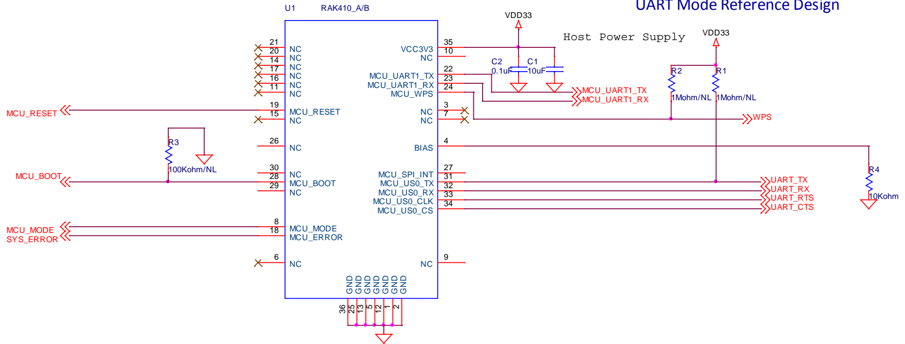
Figure 3-2-1 : RAK410 Module Peripheral Design Reference
