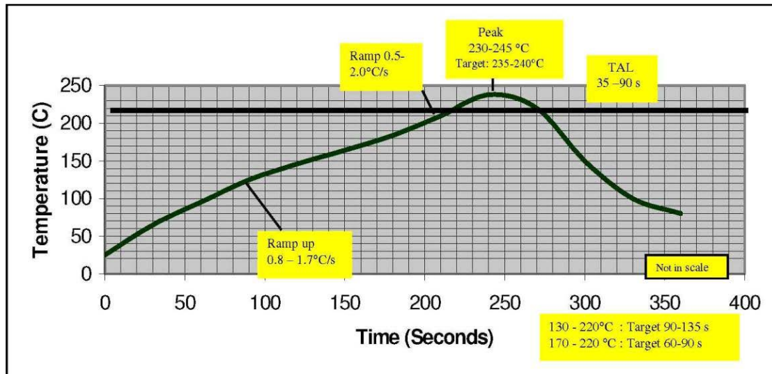
Figure 3-3-1: Reflow Profile
