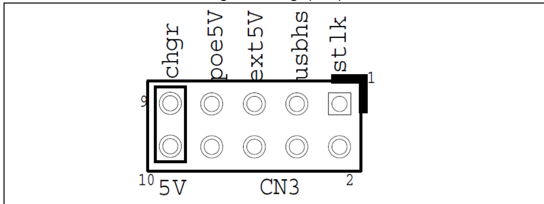
Figure 11. chgr (CN3)
