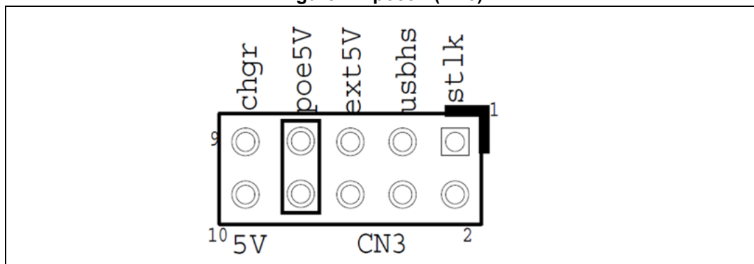
Figure 12. poe5V (CN3)
