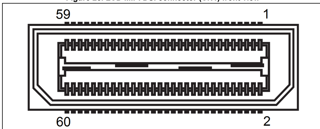
Figure 25. LCD MIPI DSI connector (CN1) front view
