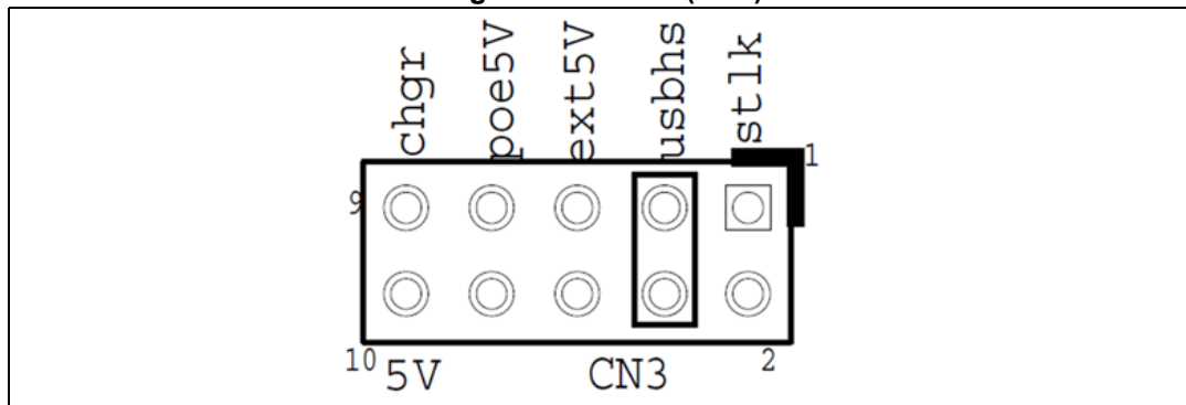
Figure 14. usbhs (CN3)
