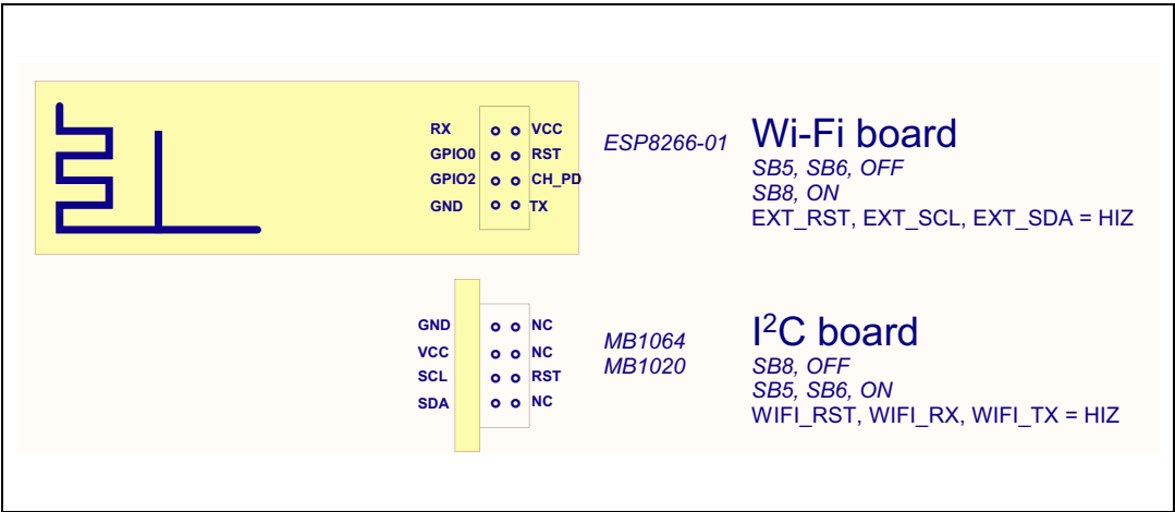
Figure 22. Wi-Fi® and I²C extension connector (CN2) front view
