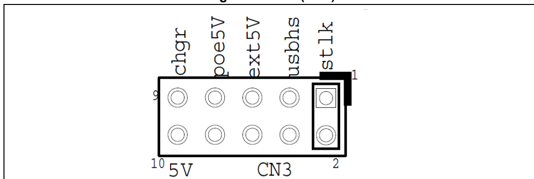
Figure 13. stlk (CN3)
